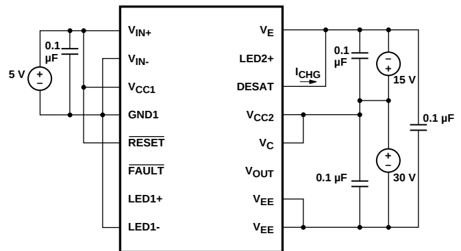
Figure 41. I CHG Test Circuit.
