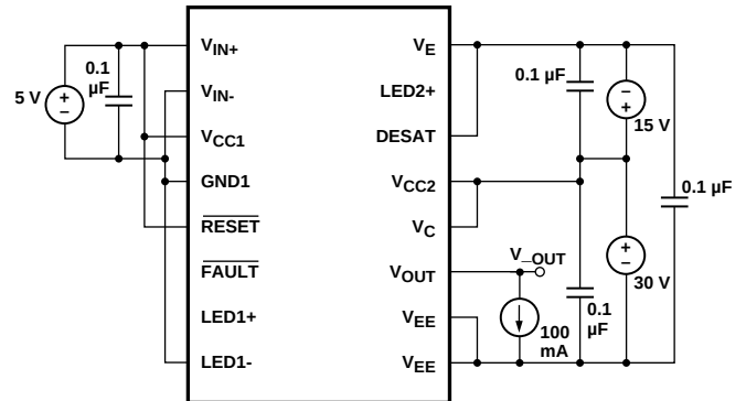
Figure 35. V_{\text{OH}} Test Circuit.
