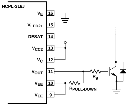
Figure 65. Output Pull-Down Resistor.
