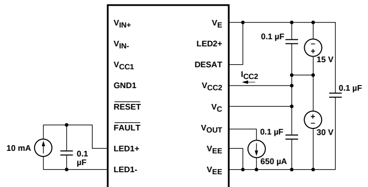
Figure 39. I CC2H Test Circuit.
