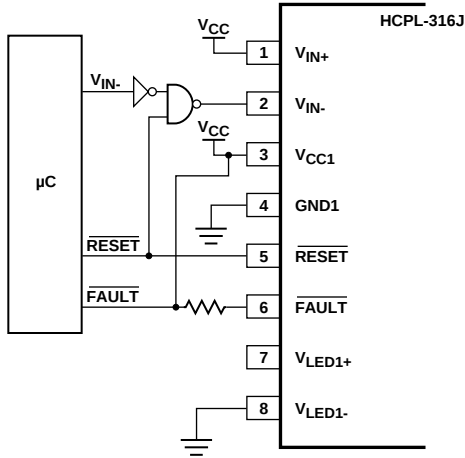
Figure 73c. Safe Hardware Reset for Inverting Input Configuration (Automatically Resets for Every V_{IN-} Input).
