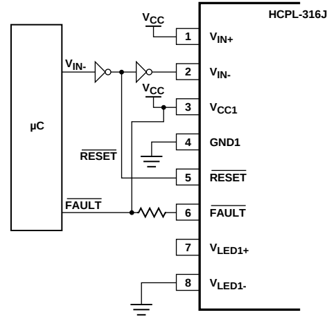
Figure 73d. Safe Hardware Reset for Inverting Input Configuration.
