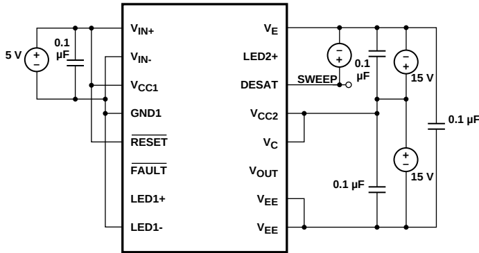
Figure 44. DESAT Threshold Test Circuit.
