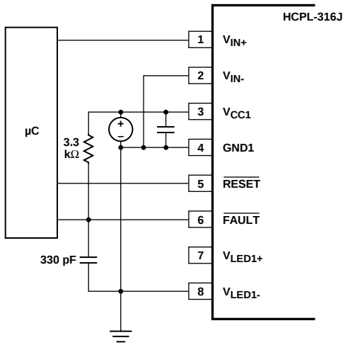
Figure 67. \overline{\text{FAULT}} Pin CMR Protection.
