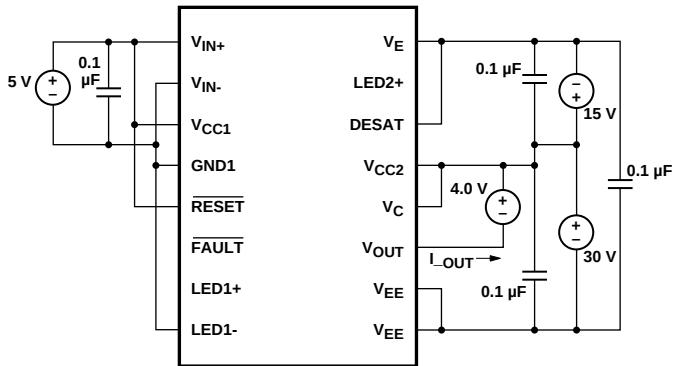
Figure 32. I_{\text{OH}} Test Circuit.
