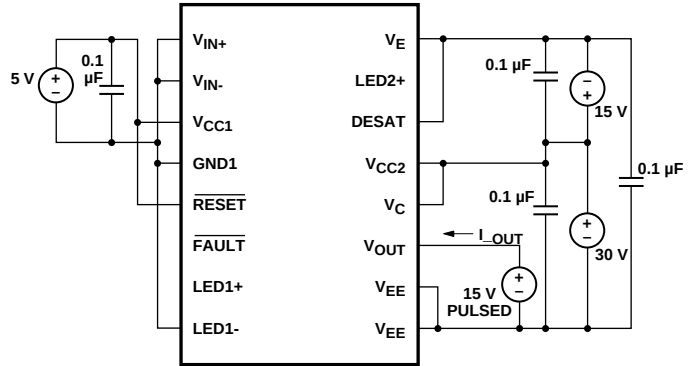
Figure 33. I_{\text{OL}} Pulsed Test Circuit.
