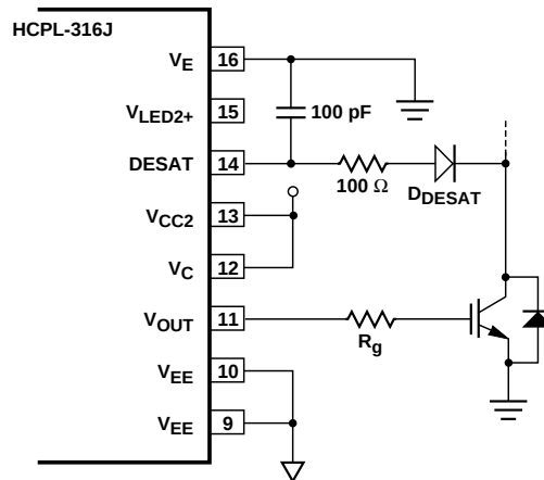
Figure 66. DESAT Pin Protection.
